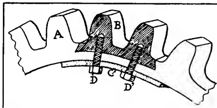
Fig. 1—Showing method of replacing damaged gear teeth
